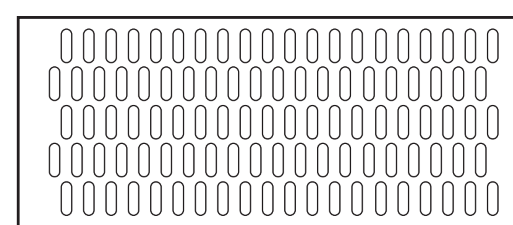
EGP130 customized suction-hole type Type:5F Customized type
